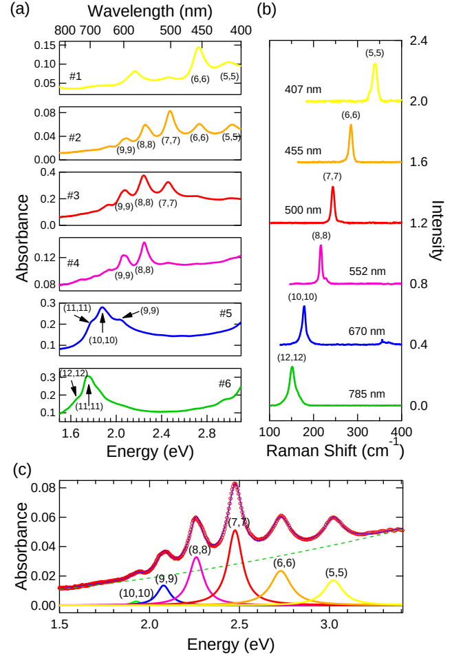
FIG. 7: (a) Optical absorption spectra of armchair-enriched SWCNT suspensions, corresponding to the samples identified in Fig. 4. The main absorption features move toward higher energy (shorter wavelength) with decreasing SWCNT diameter. (b) Associated single-line resonant Raman radial breathing mode spectra for each enriched sample, further confirming the armchair enrichment of these samples and the peak assignments in absorption. (c) Resulting fit (thin purple line) of the optical absorption spectrum of armchair-enriched sample #2 (HiPco HPR 189.2, red open circles) to a sum of six Lorentzian peaks (thick, multi-color peaks), one for each armchair (10,10) through (5,5), on top of an absorption baseline (dashed green line). Reproduced from Reference 57.
