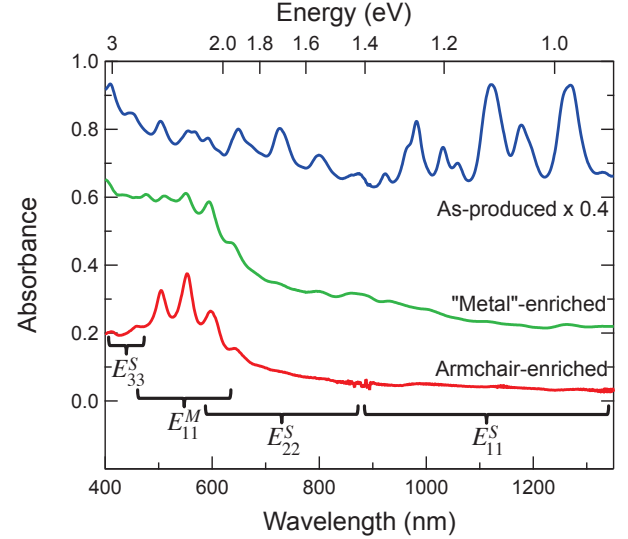
FIG. 6: Optical absorption of three HiPco nanotube suspensions studied: unsorted (AP-SWCNT, blue, top), “metal”-enriched (ME-SWCNT, green, middle), and armchair-enriched (AE-SWCNT, red, bottom). Note ME-SWCNT and AE-SWCNT show significant suppression of features due to \nu = \pm 1 SWCNTs as compared to AP-SWCNT, indicating the elimination of \nu = \pm 1 species and hence \nu = 0 enrichment by the DGU process. Reproduced from Reference 78.
