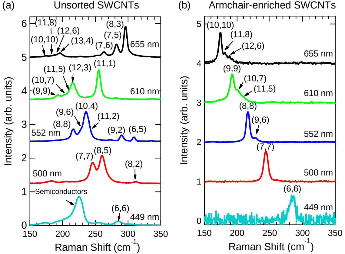
FIG. 11: Selected Raman spectra taken from data contained within Fig. 9 and 10 comparing (a) before and (b) after DGU, showing evidence for the enrichment of (a) “metallic” \nu = 0 nanotubes, and in particular, (b) armchair, or (n,n) , carbon nanotubes. Adapted from Reference 119.
