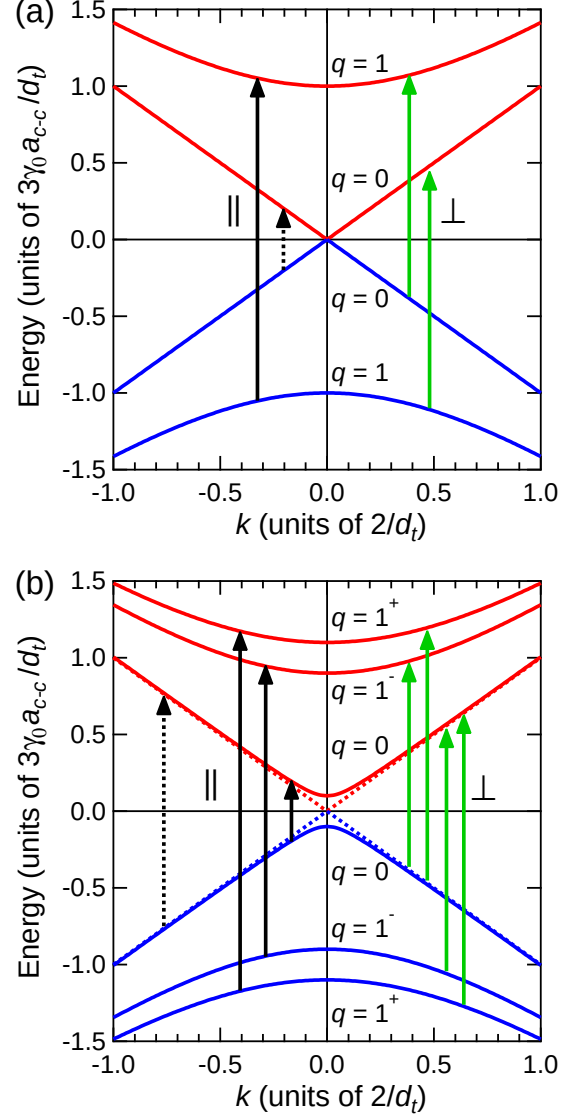
FIG. 1: Electronic band structure for (a) armchair or (n, n) and (b) non-armchair, \nu = 0 SWCNTs, where n \neq m [i.e., (n, m) ], showing both the massless, linear ( q = 0 ) and massive, hyperbolic ( |q| \geq 1 ) bands. Note that in case (b) for non-armchair \nu = 0 species, the q = 1 bands split into q = 1^+ and 1^- bands due to trigonal warping. Also, the massless q = 0 bands become massive in the vicinity of k = 0 due to the curvature-induced band gap. Valence (conduction) bands are indicated in blue (red). Solid black (green) arrows indicate allowed optical transitions for electric polarization parallel (perpendicular) to the nanotube axis. Black dashed arrows indicate forbidden optical transitions.
