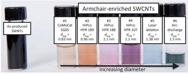
FIG. 4: Pictures of armchair-enriched SWCNT suspensions. The black, “as-produced” vial on the left is typical of unsorted, SWCNT materials. On the right, various armchair-enriched samples with different diameters exhibit different, distinct colors. Reproduced from Reference 57.
