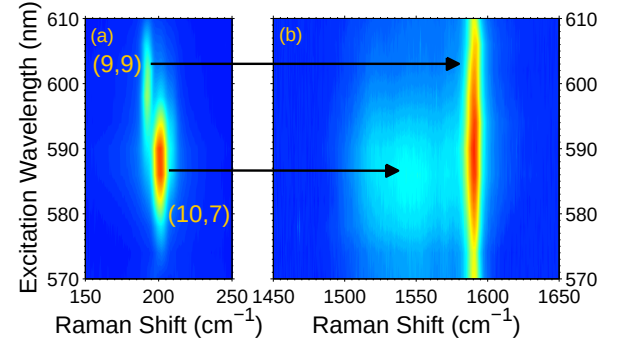
FIG. 15: Raman intensity for AE-SWCNT taken as a function of Raman shift and excitation wavelength for family 2n+m = 27 . (a) RBM region where two clear RBMs due to the (9,9) and (10,7) are observed. (b) Corresponding G-band region where only the G^+ peak is observed when resonating primarily with the (9,9) and the appearance of the broad G^- coincides with the maximum of the (10,7) RBM. Reproduced from Reference 78.
