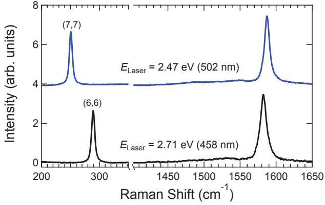
FIG. 17: Resonant Raman spectra for single-chirality armchair SWCNT samples produced by the DNA-based IEX method, taken at excitation wavelengths 502- and 458-nm. Because of the extremely singular purity of these samples, a single G^+ peak is observed due to the armchair species (7,7) and (6,6), respectively. Adapted from Reference 56.
