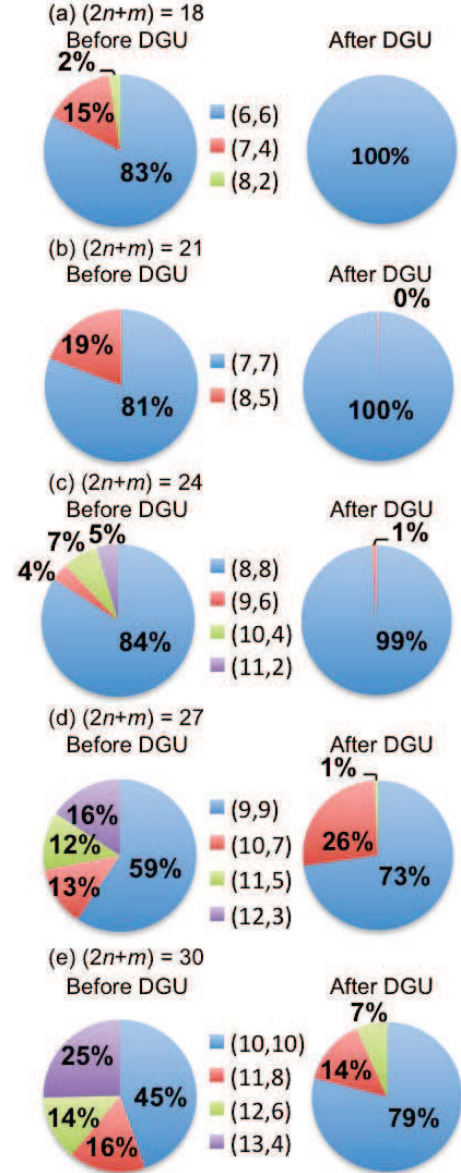
FIG. 13: Comparison of the relative abundances of \nu = 0 species in HiPco SWCNT material, before DGU (unsorted) and after DGU (armchair-enriched), as determined by resonant Raman scattering. (n, m) species are grouped together by 2n+m family, (a)-(e) corresponding to families 18, 21, 24, 27 and 30, respectively.
