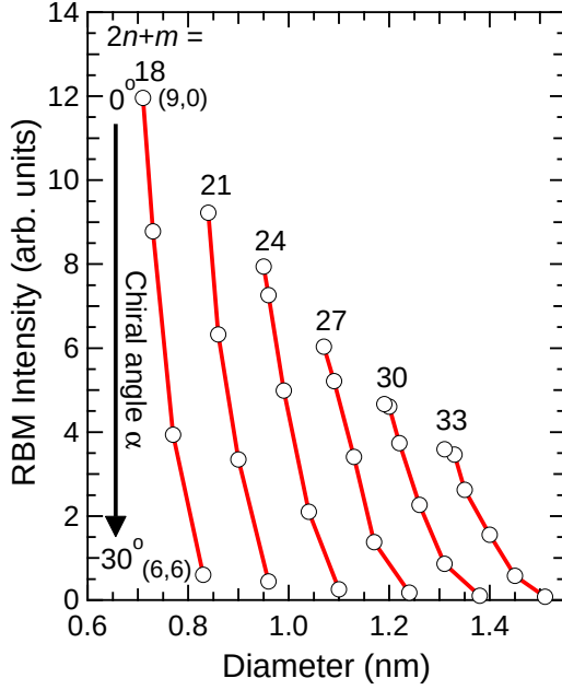
FIG. 12: Calculated RBM Raman intensities 129 for \nu = 0 SWCNT species as a function of nanotube diameter and chiral angle, with members of the same 2n+m family grouped together. Clearly, RBM Raman intensity increases with decreasing nanotube diameter and chiral angle with armchair (zigzag) species having the smallest (largest) RBM intensities for a given 2n+m family.
