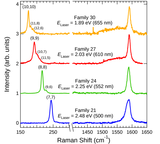
FIG. 16: Selected resonant Raman spectra for AE-SWCNT taken at excitation wavelengths 655-, 610-, 552-, and 500-nm, where resonance primarily occurs with armchair species (10,10), (9,9), (8,8), and (7,7), respectively. In each case, the G-band reflects contribution mainly from the G^+ peak only. Reproduced from Reference 78.
