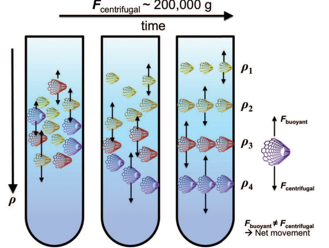
FIG. 3: Illustration of the density gradient ultracentrifugation method as applied to the separation of SWCNTs. SWCNTs of different mass density (represented by different color tubes) are loaded into a centrifuge tube containing a mass density gradient where a strong centrifugal field is applied. Due to a competition between the applied centrifugal force and the resultant opposing buoyant force, SWCNTs migrate through the gradient in space until equilibrium is reached and the forces are balanced. At this point, the SWCNTs have arrived in a region in the gradient possessing their respective mass density.
