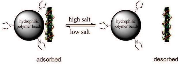
FIG. 5: Anion-exchange chromatography separation of DNA-SWCNTs. Anion exchange columns are packed with micro-sized polymer or silica beads that are surface-grafted with positively charged functional groups. DNA-SWCNTs injected into the column can be either adsorbed on the beads or remain free, depending on the concentration and chemical identity of the salt in the mobile phase. The equilibrium is also dependent on SWCNT structure, leading to fractionation of DNA-SWCNTs when they are eluted from the column by a salt gradient. By tailoring specific ssDNA strands to form ordered structures only on a specific (n, m) SWCNT surface, preferential adsorption and retention can be achieved leading to single-chirality samples.
