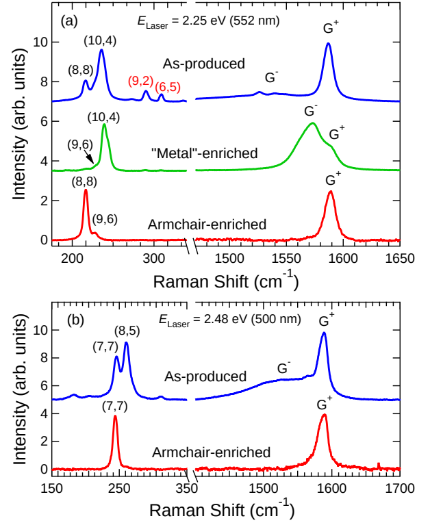
FIG. 14: Raman spectra of RBM and G-band for AP-SWCNT, ME-SWCNT, and AE-SWCNT samples taken at excitation wavelengths (a) 552 nm and (b) 500 nm where SWCNTs from families 2n+m = 24 and 21 , respectively, are primarily probed. In both sub-figures, appearance of the broad G^- feature corresponds to resonance with non-armchair species such as (10,4) in ME-SWCNT in (a) and (8,5) in AP-SWCNT in (b). In the case of singular resonance with armchair species [(8,8) and (7,7)], a single and narrow G^+ peak is observed. Reproduced from Reference 78.
