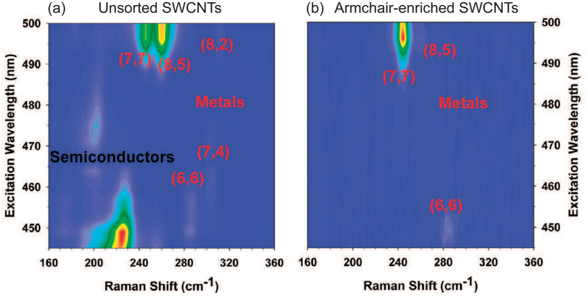
FIG. 10: Resonant Raman scattering RBM intensity contour plots of (a) unsorted and (b) metal-enriched HiPco SWCNT samples taken over an excitation range of 440-500 nm. Again, Raman intensity excitation maps of (b) clearly show enrichment of armchair carbon nanotubes relative to (a), this time for families 21 and 18. Reproduced from Reference 119.
