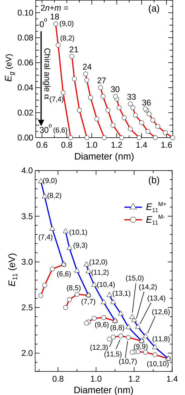
FIG. 2: Chirality dependence of the curvature-induced gap and trigonal-warping splitting in \nu = 0 or “metallic” SWCNTs. (a) A plot of calculated curvature-induced gap as a function of nanotube diameter with members of the same 2n+m family grouped together using Eq. (3). (b) A plot of predicted E_{11} optical transition energies as a function of nanotube diameter with members of the same 2n+m family grouped together for \nu = 0 SWCNTs. 48 Upper-branch E_{11}^{M+} transitions are labeled in blue and lower-branch E_{11}^{M-} transitions are labeled in red. The energy splitting between upper and lower branches is caused by trigonal warping. Both curvature-induced gap and trigonal-warping splitting are zero for armchair species and maximum for (3n, 0) zigzag species.
