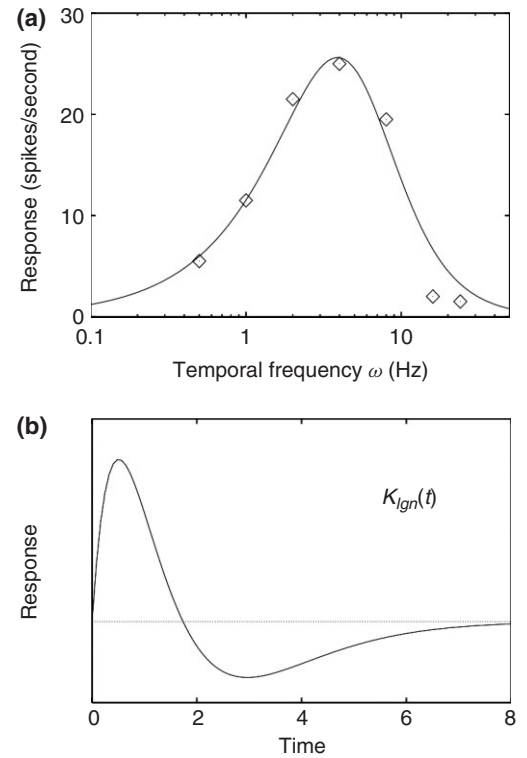
FIGURE 5 | Temporal predictive coding in the lateral geniculate nucleus (LGN). (a) Comparison between theoretically predicted temporal tuning curve (solid curve) and experimental data (points) in the LGN. 37 The predicted curve is generated from Eq. 11 with \omega_c = 5.5 Hz. (b) Temporal receptive field derived from (a) (Reprinted with permission from Ref 12. Copyright 1995 Informa PLC). Note the similarity to the temporal predictive coding filter in Figure 2(c).
