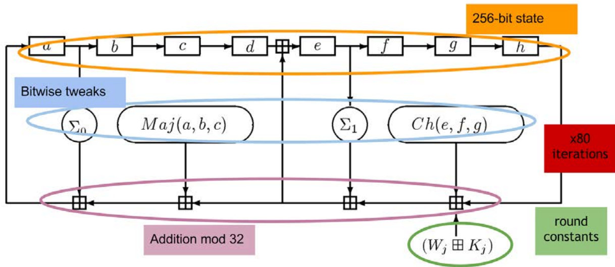
Figure 5.5 : The structure of SHA-256. This is one round of the compression function.
