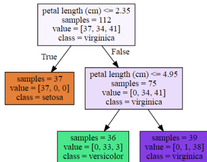
max_depth = 2
