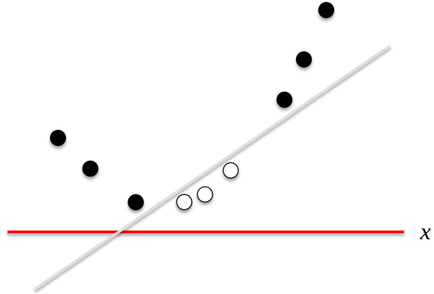
Feature space
