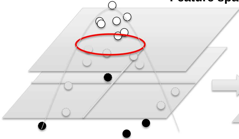
Feature space
